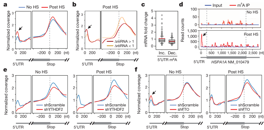
Figure 2 | Altered m 6 A profiles in MEF cells in response to heat shock stress. a , Metagenes profiles of m 6 A distribution across the transcriptome of cells before or 2 h after heat shock (42 °C, 1 h). Black arrow indicates the m 6 A peak in the 5'UTR region. b , Transcripts are stratified by different expression levels after heat shock stress, followed by metagenes profiles of m 6 A distribution. c , A box plot depicting fold changes of mRNA levels after heat shock for transcripts showing increased or decreased m 6 A modification in the 5'UTR.
