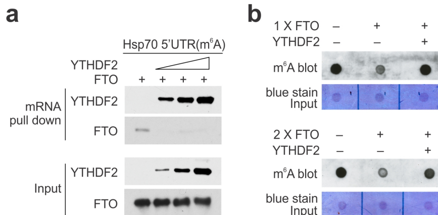
Extended Data Figure 6 | Direct competition between YTHDF2 and FTO in m 6 A binding. a , Synthesized mRNA with m 6 A was incubated with FTO (2 µg) in the presence of an increasing amount of YTHDF2 (0, 0.5, 1 and 2 µg), followed by RNA pull-down and immunoblotting. b , Synthesized
