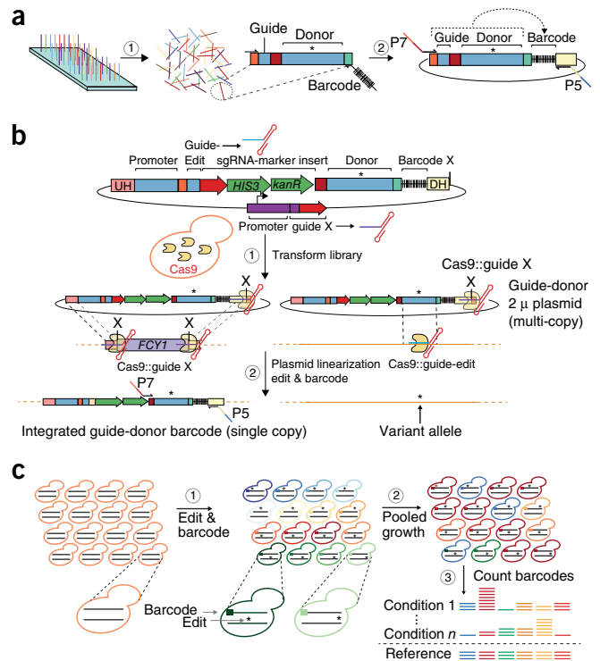
Figure 1 The MAGESTIC pipeline for multiplexed precision genome editing. (a) Linking guide–donors to short DNA barcodes. (1) A complex pool of array-synthesized oligonucleotides encoding guide–donors is amplified and cloned to generate the step 1 library. The reverse primer introduces a semi-random 31-mer barcode into each ligation product, and (2) NGS enables sequence validation and computational mapping of each guide–donor sequence in the step 1 library to a unique barcode. (b) Insertion of the Cas9 structural guide component plus selection markers from yeast ( HIS3 ) and bacteria ( kanR ) in between the guide and donor. (1) This final step 2 library is transformed into yeast cells such that the vast majority of transformants uptake a single plasmid, which accumulates to a high-copy number. Each cell harbors a barcode integration locus with a counter-selectable marker ( FCY1 ). Guide–donor plasmids harbor a second guide expression unit (guide X) to promote barcode integration, as guide X cleavage sites flank FCY1 . (2) Cas9 and guide expression results in simultaneous cleavage of the guide–donor plasmid at a guide X site adjacent to the downstream homology (DH), target site editing (right), and genomic integration of the guide–marker–donor–barcode cassette (left). (c) Library-scale genome editing and competitive growth phenotyping. (1) The guide–donor plasmids allow editing throughout the genome, while the barcode integration site is constant. (2) Pooled growth in different conditions results in enrichment or depletion of variants that affect fitness. (3) Variant fold-changes are calculated based on barcode sequencing counts in treated vs. untreated conditions.
