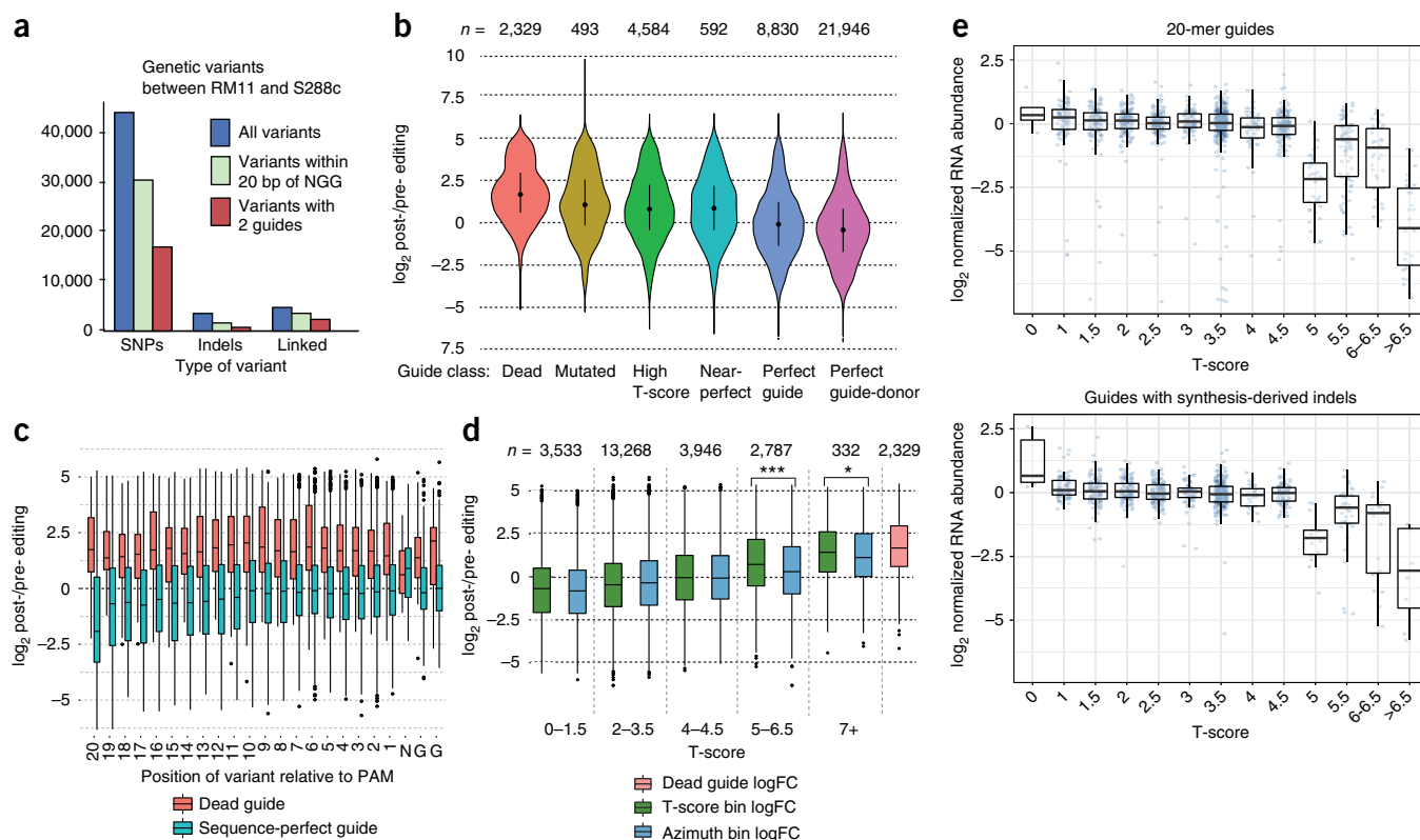
Figure 5 Global profiles of guide efficacy and mismatch tolerance for engineering of natural variants. (a) Number of individual genetic variants between RM11 and S288c. (b) \log_2 -fold change (logFC) of barcodes in each guide class post-editing vs. pre-editing (dead guides: indels within 15 bp from PAM or \geq 2 mismatches within 18 bp; mutated guides: 1 mismatch within 18 bp or indel from 16–18 bp; near-perfect: mismatches at positions 19 or 20). High T-score is defined as \geq 5 . (c) Dead and perfect guide–donor logFC by distance of the variant allele from the PAM. Variants shown in the N of the NGG consisted solely of indels or linked variants and harbor additional disruption positions upstream or downstream. (d) Boxplots of logFC by T-score bin with Azimuth score bins of the same size (one-sided Wilcoxon P -values: *0.03182, *** 8.12 \times 10^{-14} ). (e) Normalized RNA abundances as a function of T-score for sequence-perfect guides (top) and guides with synthesis-derived indels (bottom). RNA levels were determined by targeted RT-PCR of the guide RNAs and PCR of the guide DNA sequences followed by high-throughput sequencing. RNA and DNA levels were analyzed in biological triplicates and similar results were obtained with random hexamers and with a structural-guide-specific primer for reverse transcription. Box and violin plots show median value, and 25 th and 75 th quantiles. The number of barcodes ( N ) analyzed in each group is shown at the top of each plot for b and d , and in the Methods, section statistical analysis, for c .
