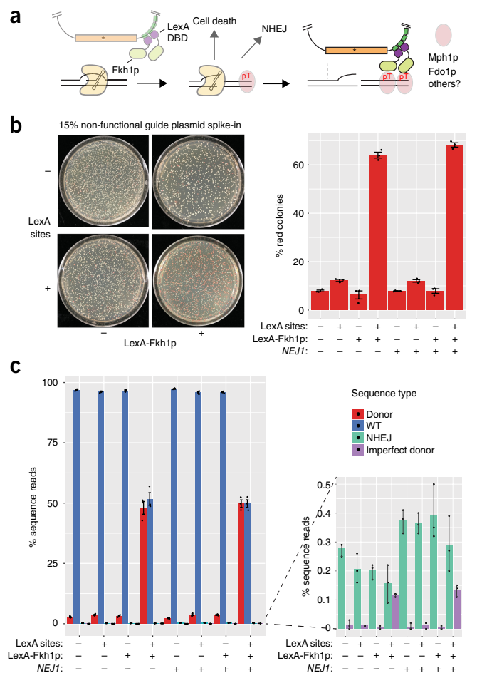
Figure 3 Active recruitment of donor DNA to Cas9-induced dsDNA breaks increases homologous recombination efficiency. (a) A protein fusion of Fkh1p to the LexA DNA-binding domain (LexA–Fkh1p) enables recruitment of donor DNA directly to dsDNA breaks (DSBs). DSBs result in the accumulation of proteins phosphorylated on specific threonine residues (pT) near the site of the break. The interaction between Fkh1p and various pT-containing proteins (including Mph1p, Fdo1p, and additional unidentified proteins) recruits LexA–Fkh1p to DSBs, which in turn recruits donor DNA via LexA binding sites on the plasmid. (b) ADE2 -guide donor plasmids with (bottom) or without (top) LexA sites were mixed with a non-functional ADE2 guide–donor plasmid at a ratio of 17:3, and transformed into a strain pre-expressing TEF1 -Cas9 with (right) or without (left) LexA–Fkh1p. Red colonies indicate cells that received a functional ADE2 guide–donor and survived editing, while white colonies represent cells that received the non-functional ADE2 guide. The bar chart depicts the mean percentage of red colonies (y axis) determined by counting three plates per condition (x axis). Error bars represent the s.d. (c) The ADE2 locus was analyzed as in Figure 2. Because ade2 is a detrimental mutation, ade2 null colonies are smaller and thus contribute slightly fewer sequence reads per colony relative to white colonies. The bar chart (left) indicates that >99.5% of the sequence is WT or perfect donor repair. The inset bar chart (right) shows the remaining <0.5% of editing events (Supplementary Table 1).
