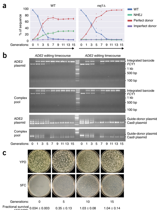
Figure 2 Simultaneous genome editing, guide–donor barcode integration, and plasmid self-destruction. (a) WT and nej1 \Delta were transformed with GAL–Cas9 and a guide–donor cassette to introduce a PTC in the ADE2 gene. Cas9 expression was induced by galactose and aliquots were harvested at the indicated generations. The ADE2 locus was analyzed by NGS and the fractions of WT sequence, NHEJ indels, and donor–DNA–directed editing (either perfect or imperfect repair) were calculated. The line graph shows the mean percentages at each generation from duplicate experiments. (b) Integration of the guide–donor barcode was assayed by amplification targeting the chromosomal barcode locus for the single ADE2 guide–donor plasmid (top) as well as a complex pool of >100,000 barcoded guide–donor plasmids (bottom). The uncropped gel image indicates an absence of detectable NHEJ indel events at the barcode locus. Self-destruction of the guide–donor plasmids was assessed by a three-primer PCR, with a common forward primer and either a guide–donor plasmid-specific primer (top band) or a Cas9–plasmid-specific primer (bottom band). (c) Cultures at the indicated generations of galactose induction were plated in quadruplicate at a density of ~1,000 cells per plate on rich medium (YPD) and FCY1 counter-selectable medium (5-FC). The fraction of surviving colonies on plates are shown. All experiments were repeated with three biological replicates starting from independent transformations of the guide–donor plasmids. (Full gel images are available in Supplementary Fig. 9.)
