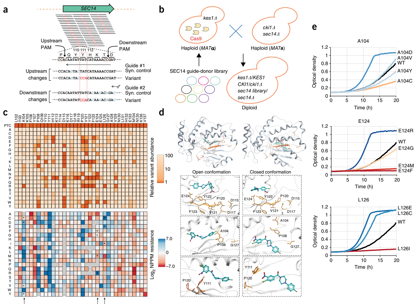
Figure 4 Saturation mutagenesis of an essential eukaryotic gene and structure-function mapping of drug resistance. (a) Synonymous-codon-spreading strategy for complete saturation mutagenesis of ORFs ( Supplementary Fig. 3 ). (b) Suppressor strategy for assaying function of Sec14p mutants. (c) Heatmaps depicting the fitness cost of each mutation in SEC14 on protein function (top) and resistance to the Sec14 small-molecule inhibitor NPPM (bottom). The normalized relative abundance of each variant in the diploid library was assessed by sequencing (top), and read counts following ~12 generations of growth in 8 \mu M NPPM versus DMSO control were used to calculate relative resistance (bottom). Rows indicate specific amino acid substitutions, and columns indicate amino acid position in Sec14. Color intensity indicates the degree to which each amino acid mutation negatively impacted Sec14 function (orange, top panel), and increased (blue) or decreased (red) Sec14 resistance to NPPM (bottom panel). The light gray blocks indicate variants with insufficient read counts. The screen was conducted in biological replicates. (d) The Sec14 \alpha -carbon backbone (gray) and the mutated window (orange), with the NPPM modeled into both the open (left) and closed (right) conformers of Sec14. Side chains critical for protein function (top panel) and NPPM resistance (middle and bottom panels) are highlighted relative to the predicted binding position for NPPM. (e) The indicated mutants were independently reconstructed and grown with 8 \mu M NPPM. OD600 was followed over 20 h of growth, with WT growth plotted as reference (black line). Growth assays were conducted in biological triplicate, which produced nearly identical results ( Supplementary Table 2 ).
