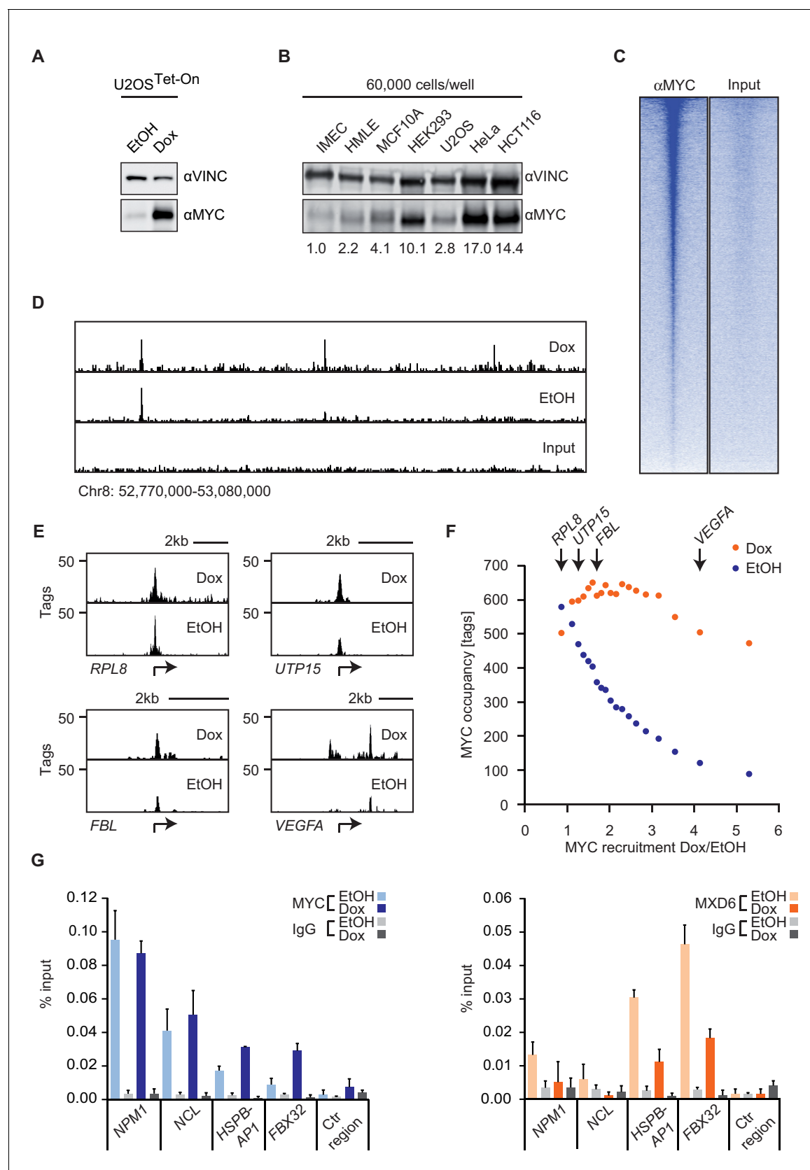
Figure 1. MYC saturates certain binding sites. (A) Immunoblot of MYC and Vinculin in U2OS Tet-On cells treated with EtOH or with 1 \mu g/ml of doxycycline. (B) Immunoblot of MYC and Vinculin in several transformed (U2OS, HeLa, HCT116) and untransformed cell lines (IMECs, HMLE, MCF10A, Figure 1 continued on next page
