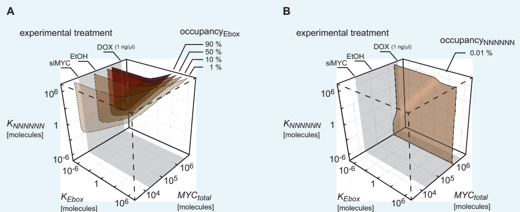
Appendix 2–figure 1. Plot shows surfaces of equal occupancy as function of dissociation constants K_{NNNNNN} and K_{Ebox} as well as total amount of MYC. Different regions of occupancy of E-boxes (A) and NNNNNN sequences (B) are shown in this parameter space. The experimentally measured range of the total amount of MYC is marked in grey. Total MYC concentrations of U2OS cells were changed by different experimental treatments as indicated on the upper axis. To simulate U2OS cells, [Ebox_{total}] = 9.3 \cdot 10^5 and [NNNNNN_{total}] = 9.5 \cdot 10^9 are assumed.
